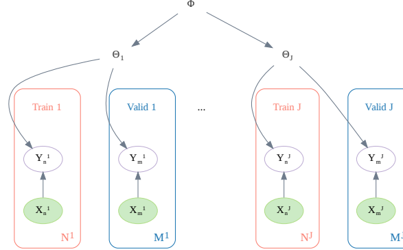
Figure 19.14: Illustration of a hierarchical Bayesian model for meta-learning. Generated by hbayes_maml.ipynb .
