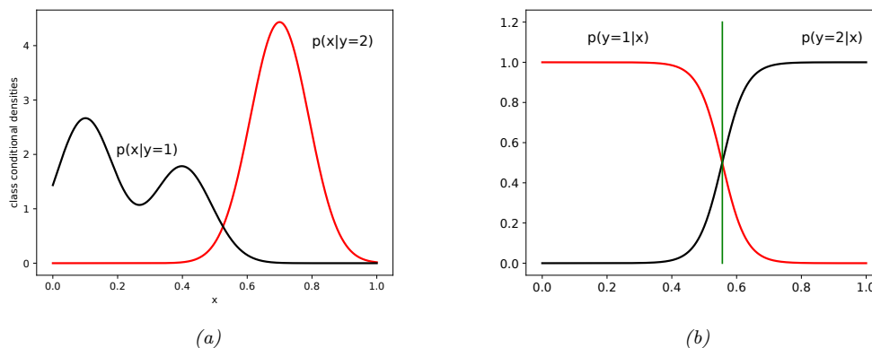
Figure 9.8: The class-conditional densities p(x|y = c) (left) may be more complex than the class posteriors p(y = c|x) (right). Adapted from Figure 1.27 of [Bis06]. Generated by generativeVsDiscrim.ipynb .
