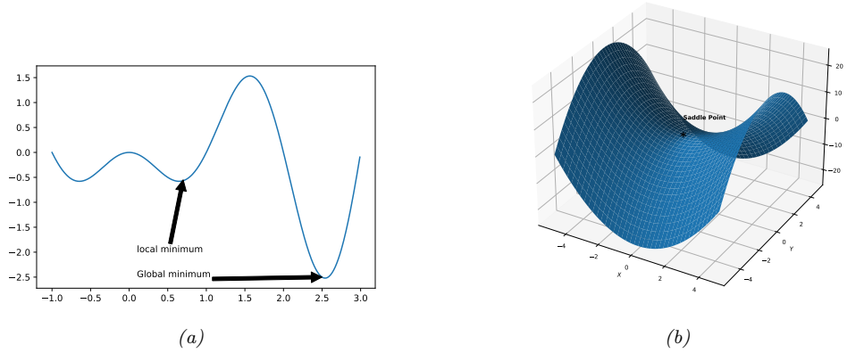
Figure 8.1: (a) Illustration of local and global minimum in 1d. Generated by extrema_fig_1d.ipynb . (b) Illustration of a saddle point in 2d. Generated by saddle.ipynb .
