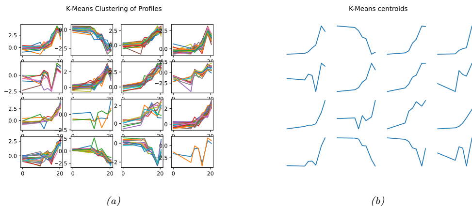
Figure 21.8: Clustering the yeast data from Figure 21.5 using K-means clustering with K = 16 . (a) Visualizing all the time series assigned to each cluster. (b) Visualizing the 16 cluster centers as prototypical time series. Generated by kmeans_yeast_demo.ipynb .
